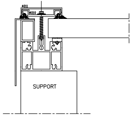
RACCORD SUPPORT
